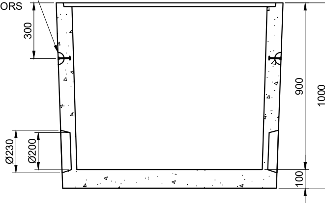
SECTION A
