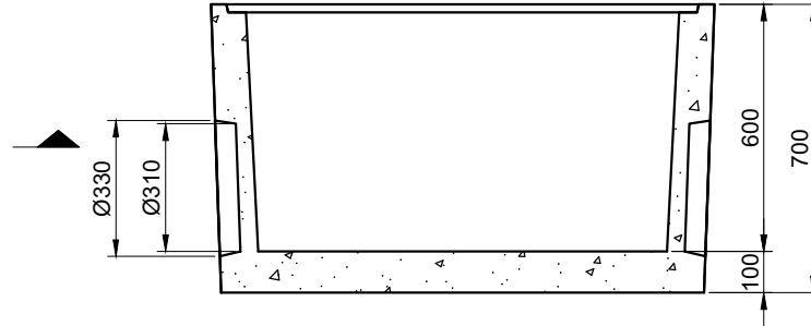
SECTION A
