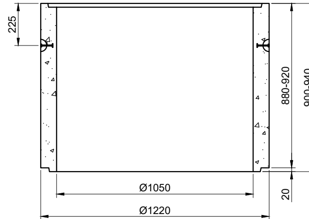
SECTION A
