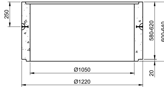
SECTION A
