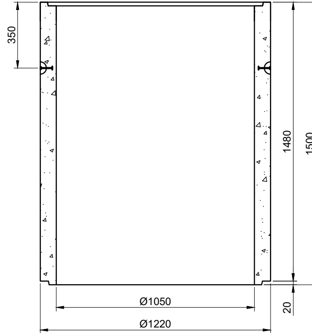
SECTION A
