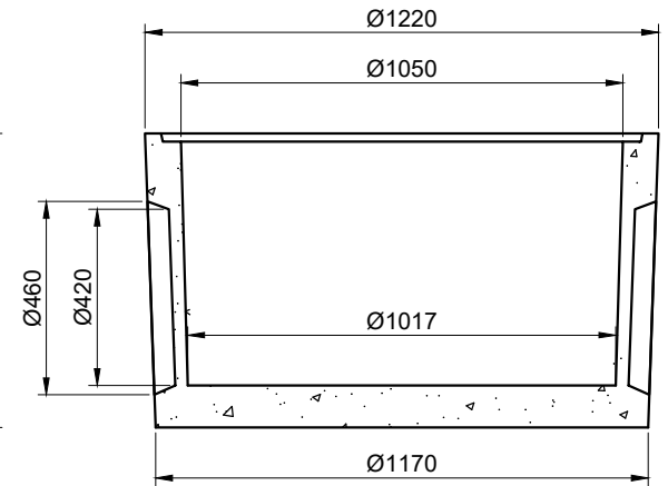
SECTION B
