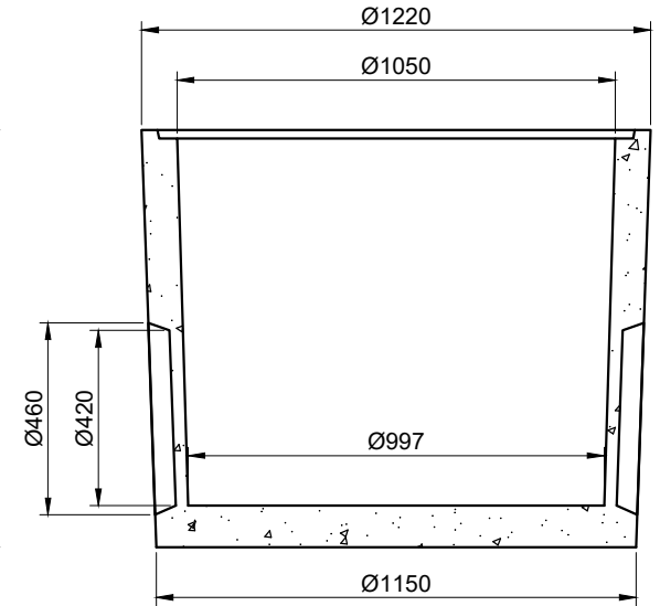
SECTION B
