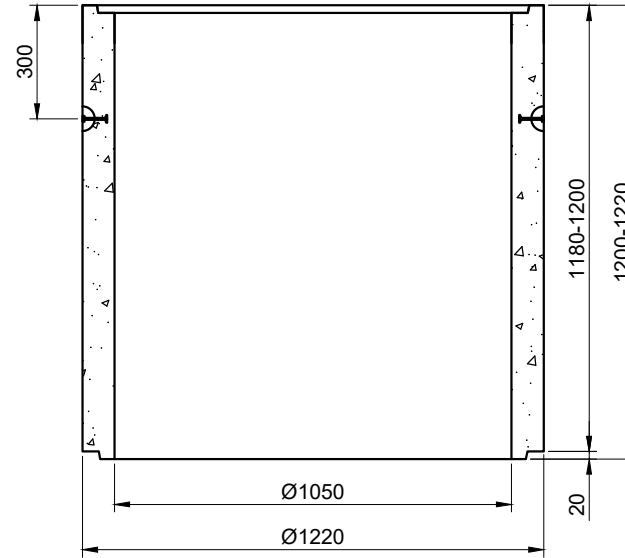
SECTION A
