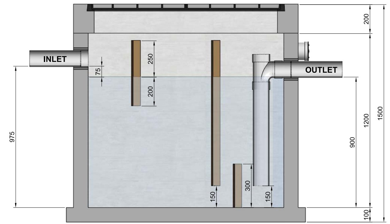
SECTION A 1000L
