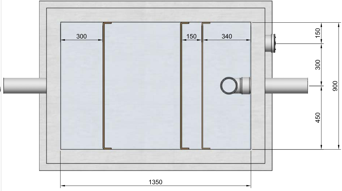
PLAN VIEW COVER REMOVED
