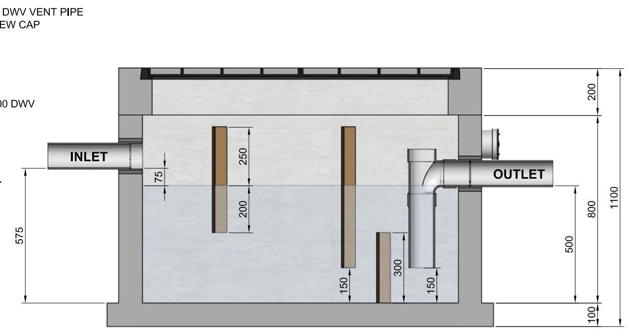
SECTION A 600L
