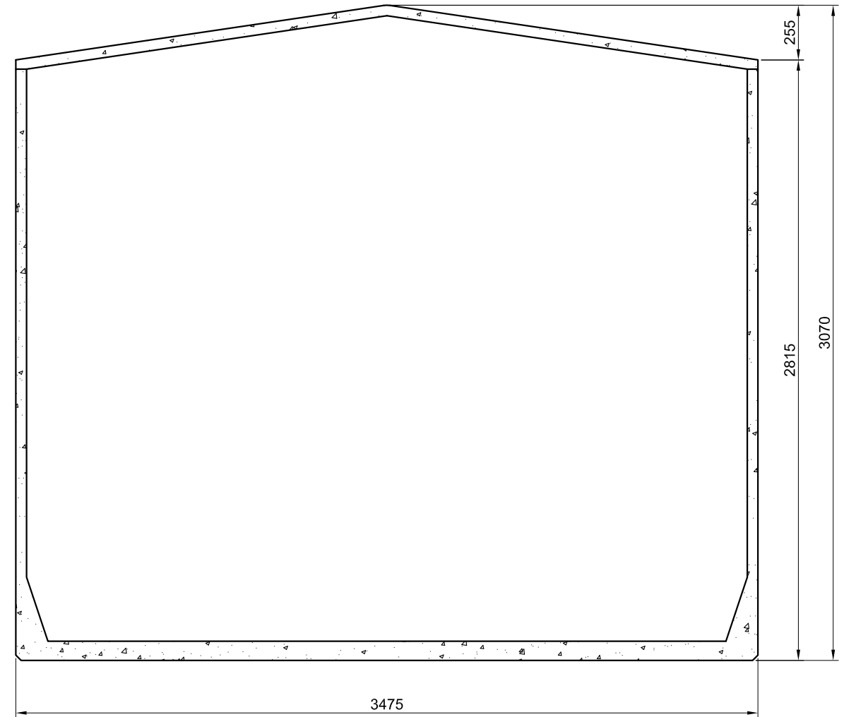
SECTION A NOT ALL DETAILS SHOWN FOR CLARITY
